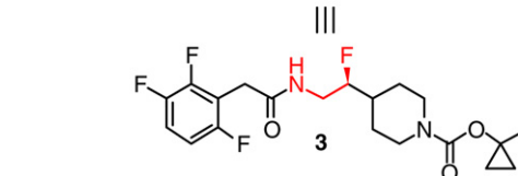
Figure 3. Averaged conformation of 3 in solution on the NMR timescale.
