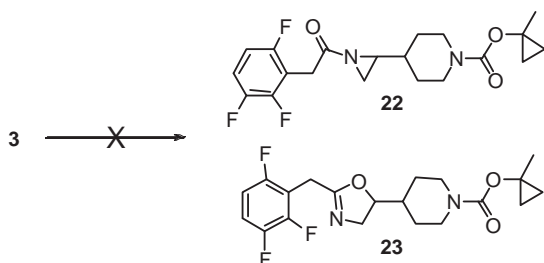
Scheme 2. Attempts of intramolecular displacement of fluorine in 3 .
