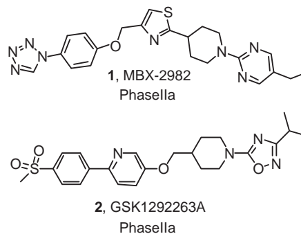
Figure 1. Structure of some known GPR119 agonists in the clinic.
