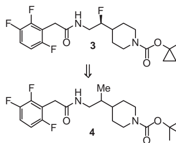
Figure 2. 2-(2,3,6-Trifluorophenyl)acetamide GPR119 agonists.
