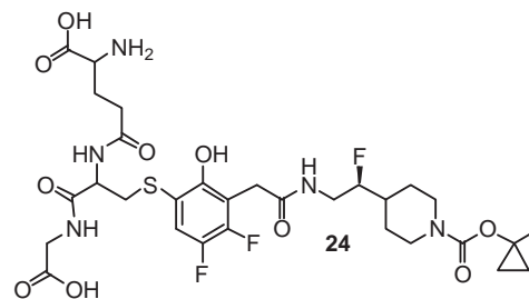
Figure 4. Representative structure of glutathione adduct 24 .
