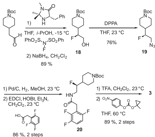
Scheme 1. Synthesis of compound 3 .
